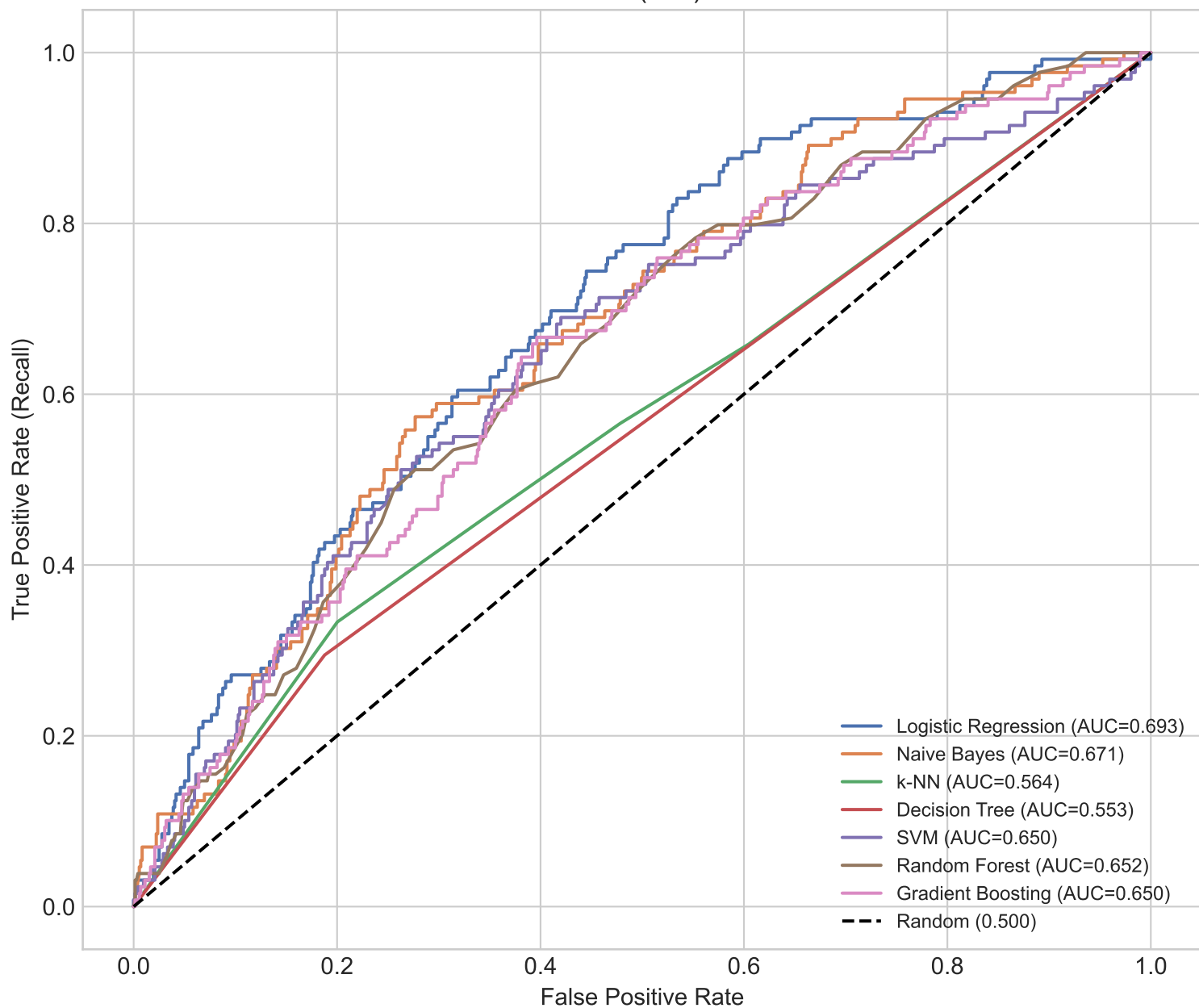
ROC curves (test) - scaled
